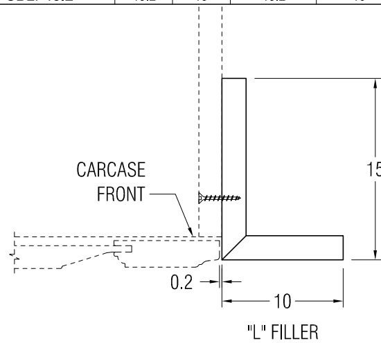
"L" FILLER DETAILS (TOP VIEW)
