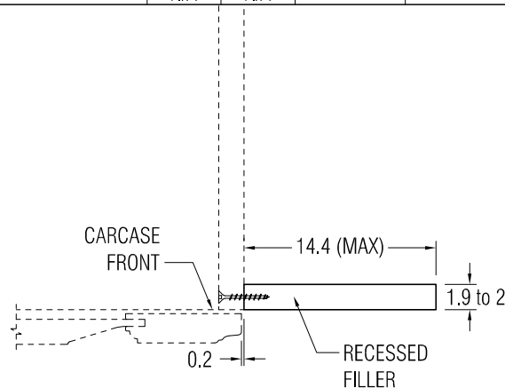
RECESSED FLUSH w/ CARCASE FILLER DETAILS (TOP VIEW)
