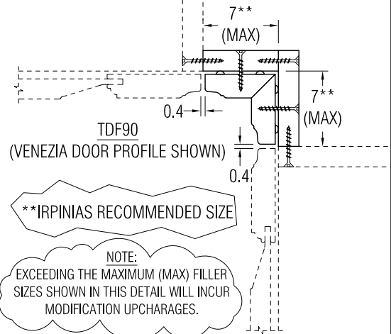
90 DEGREE DOOR DESIGN FILLER DETAILS (TOP VIEW)
