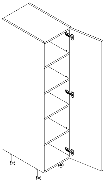
TWO SET BACK GABLES (RIGHT HINGE SHOWN)
