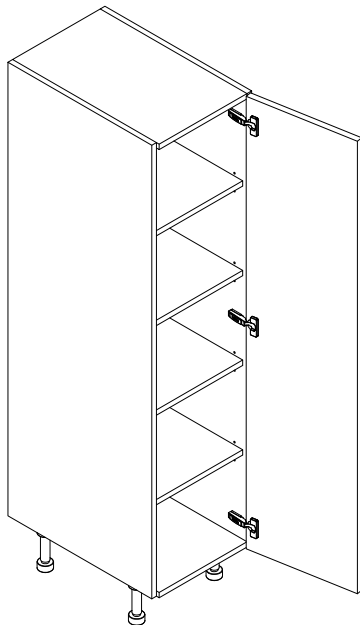
ONE SET BACK GABLE (RIGHT HINGE SHOWN)
