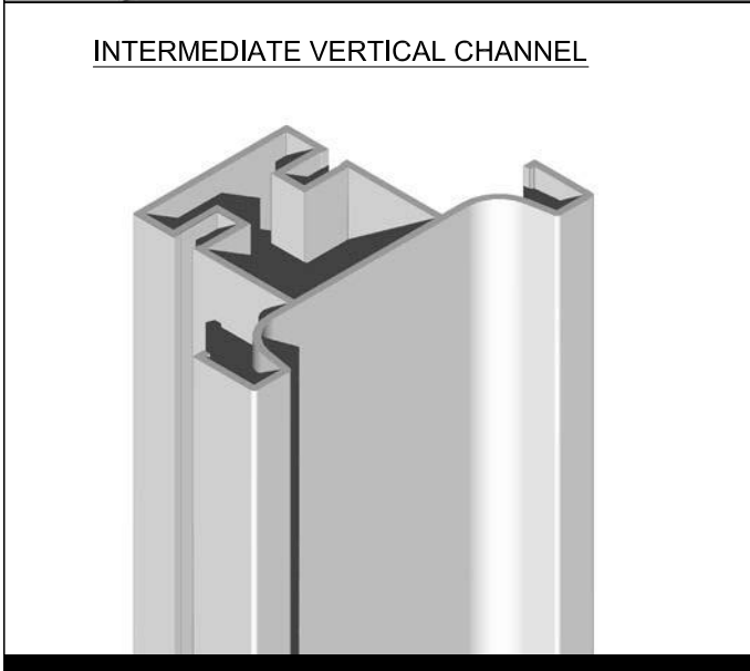
INTERMEDIATE VERTICAL CHANNEL (SECTION)
