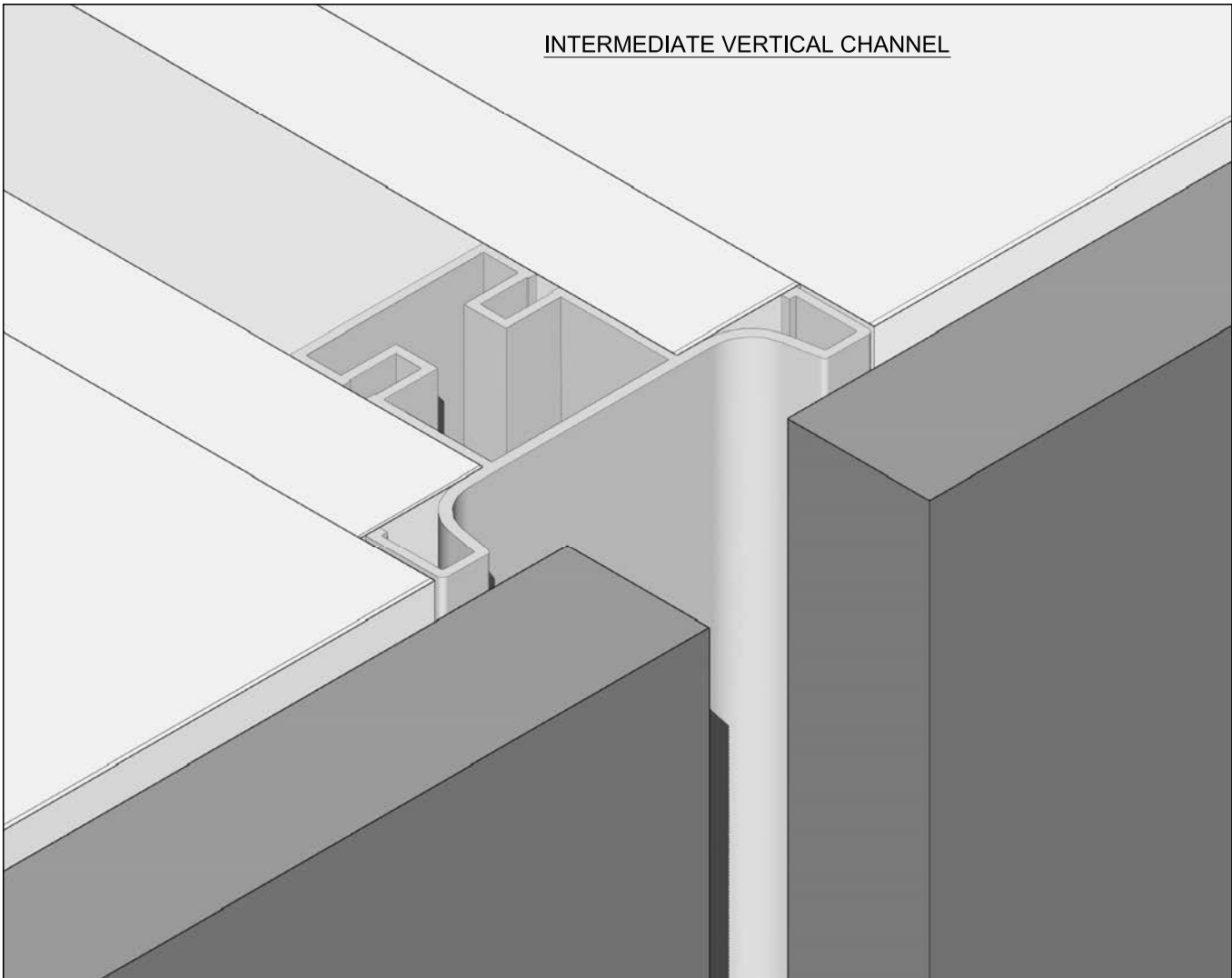
INTERMEDIATE VERTICAL CHANNEL
