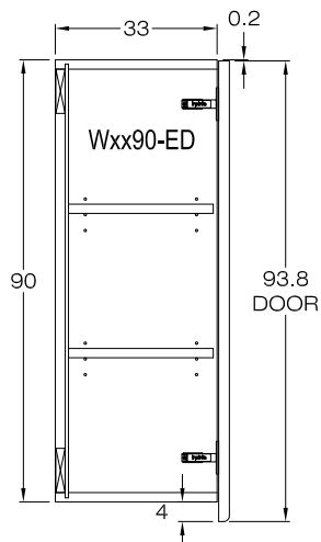
WALL 33cm DEEP SECTION DETAILS
