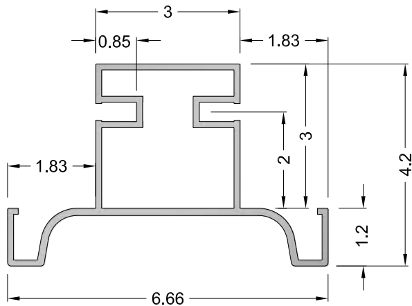
INTERMEDIATE VERTICAL CHANNEL (SECTION)
