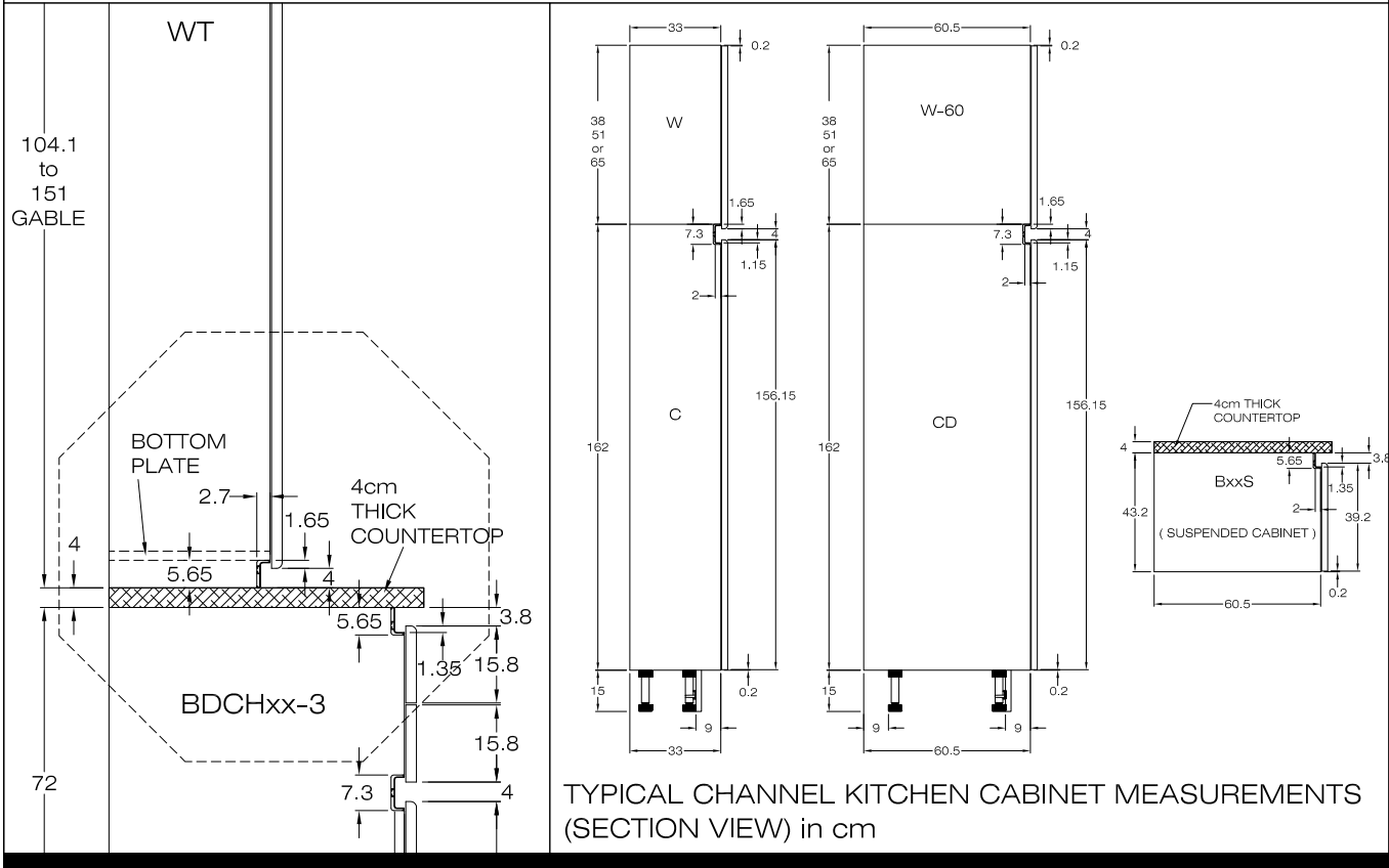
TYPICAL CHANNEL KITCHEN CABINET MEASUREMENTS in cm (SECTION VIEW)
