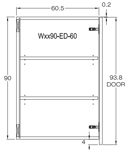
WALL 60.5cm DEEP SECTION DETAILS
