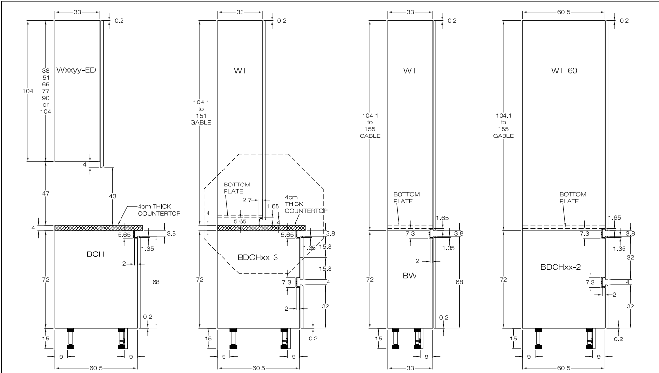
TYPICAL CHANNEL KITCHEN CABINET MEASUREMENTS in cm (SECTION VIEW)
