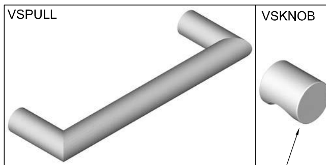
VSPULL - ALUMINUM 9.6cm C-C; 10.9cm L X 1.1cm W X 3.3cm HH, ORDER CODE: VSPULL
