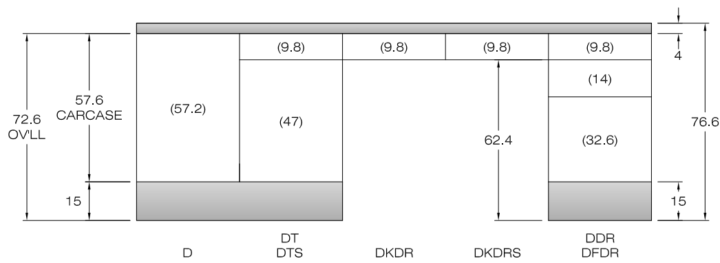
TYPICAL DESK HEIGHTS in cm (ELEVATION VIEW)
