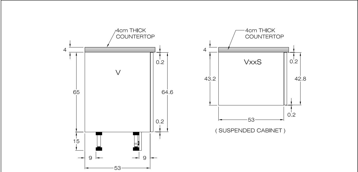
TYPICAL VANITY CABINET MEASUREMENTS in cm (SECTION VIEW)
