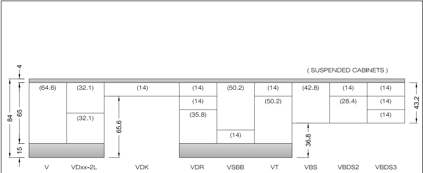
TYPICAL VANITY CABINET HEIGHTS in cm (ELEVATION VIEW)
