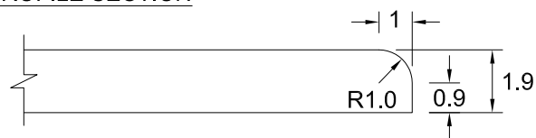
PROFILE SECTION
