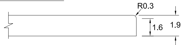
PROFILE SECTION
