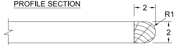
SHALLOW DRAWER FRONT SECTION
