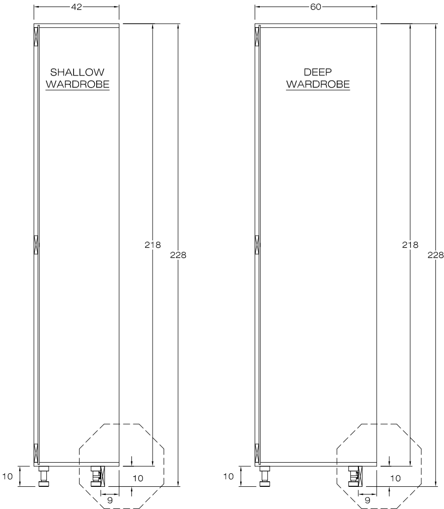
TYPICAL WARDROBE CABINET MEASUREMENTS in cm (SECTION VIEW)
