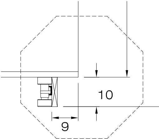
TYPICAL WARDROBE TOEKICK MEASUREMENTS in cm (SECTION VIEW)
