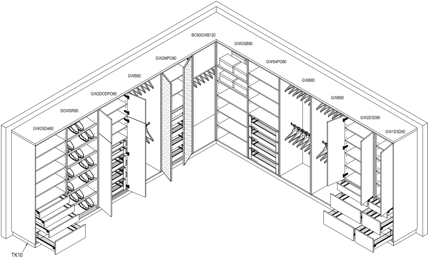
SAMPLE #2 WARDROBE LAYOUT w/ INTIVO DRAWERS AND PULL OUTS SHOWN
